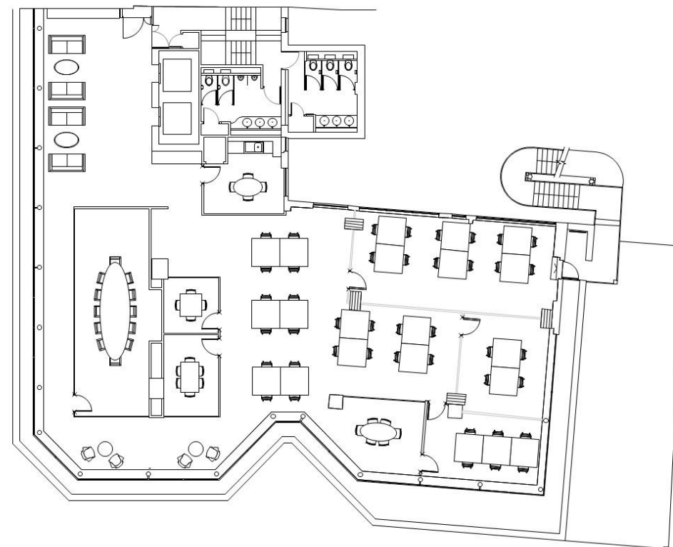
5 th floor Floorplan
