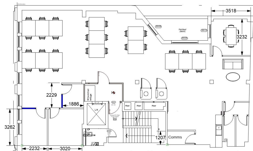
Example Floorplan:
